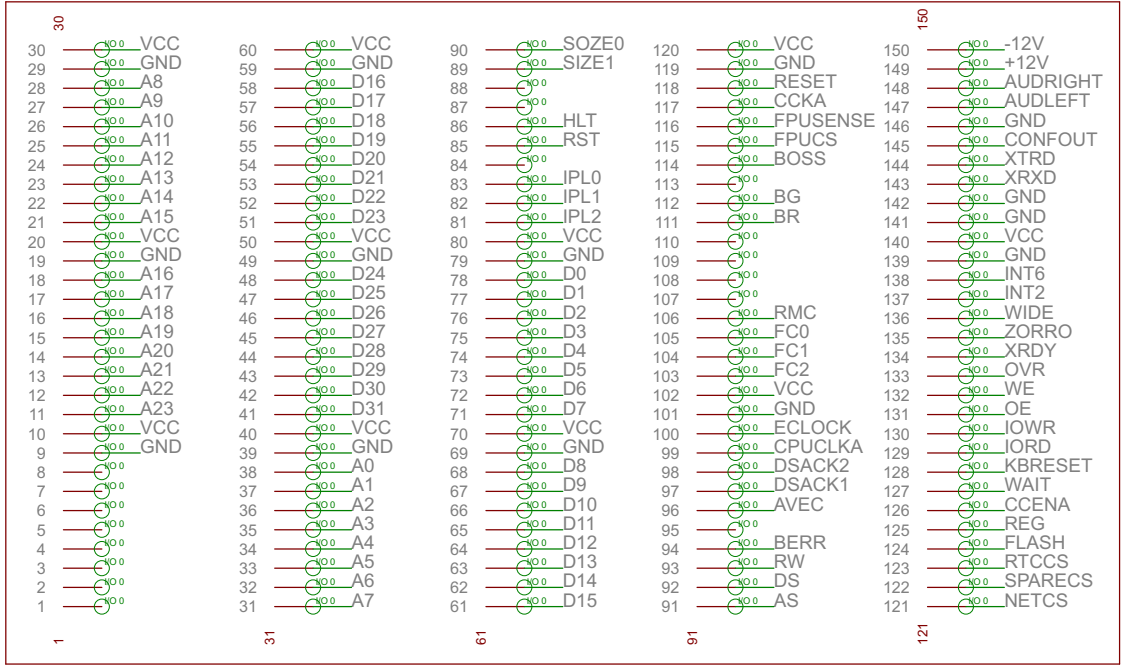
Amiga 1200 Connector 150 pin
